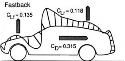
Fig 4.8 Aerodynamic lift and drag forces with different vehicle styles.
